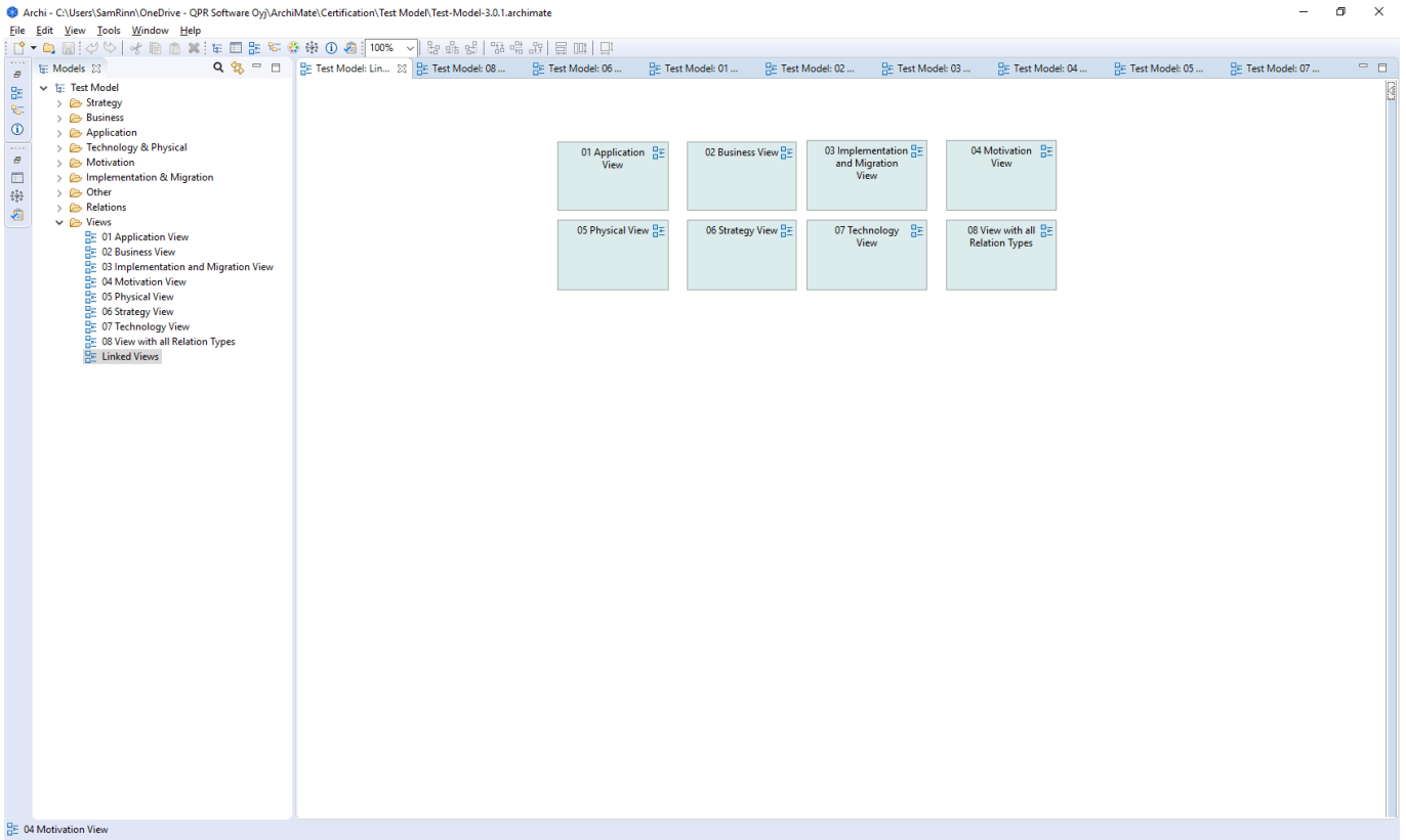
Linked Views
