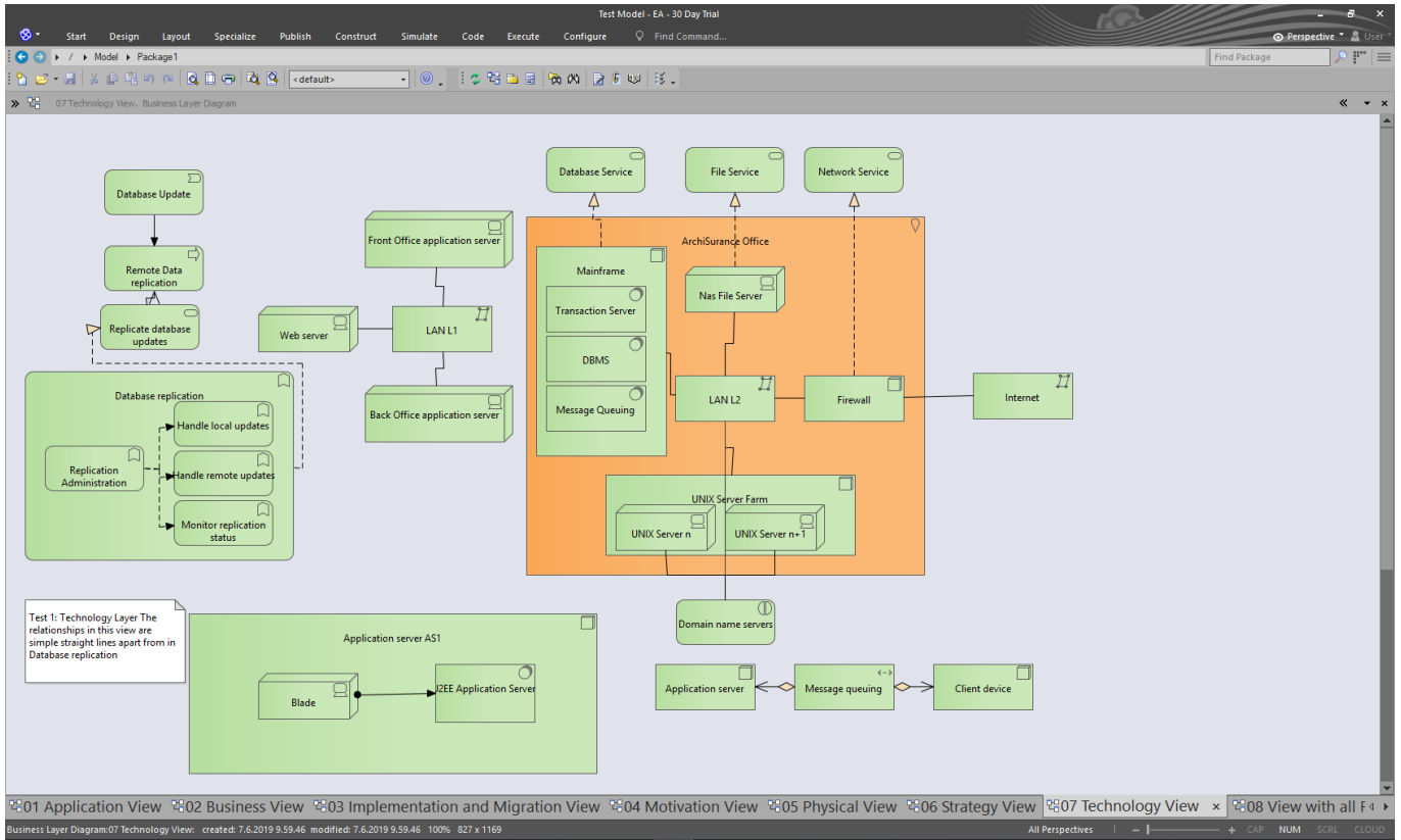
07 Technology View
