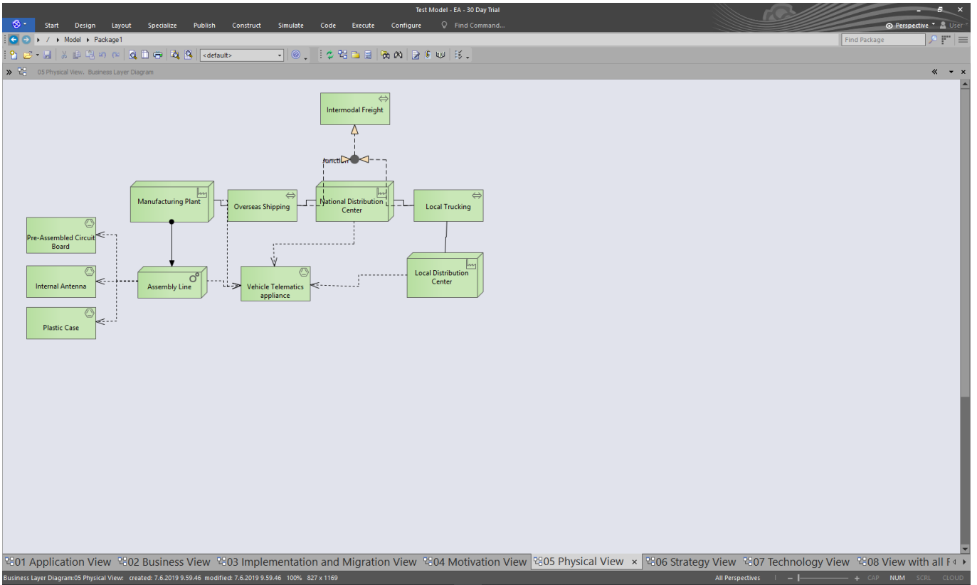
05 Physical View
